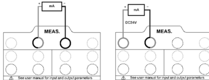
Figure 8 Current measurement
