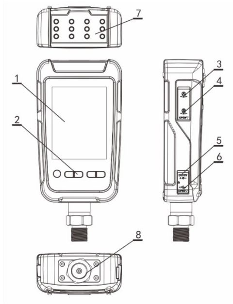
Figure 1 Basic Structure
